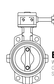
BL301T Wafer Teflon Lined Lever Op Size : 40~150mm (1½"~6")
