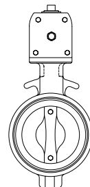
BE301 Wafer, Pneumatic Op Size : 40~1000mm (1½"~40")
